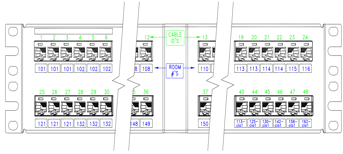
Patch Panel Labeling Diagram
