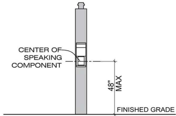
ELEVATION C12-D8
